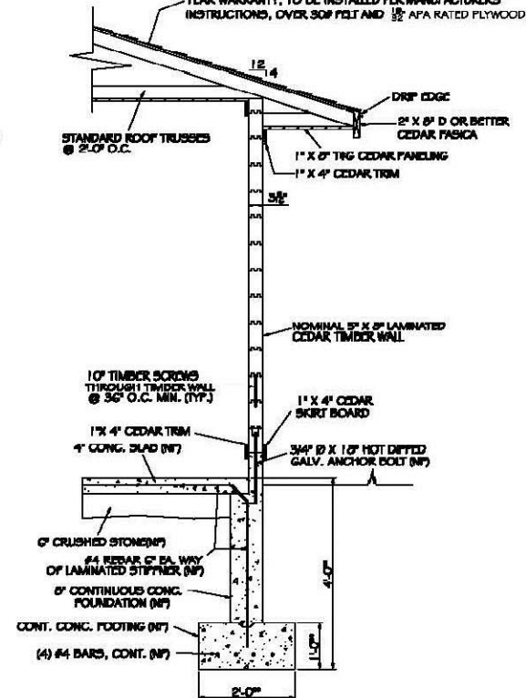
TIMBER WALL CROSS SECTION
