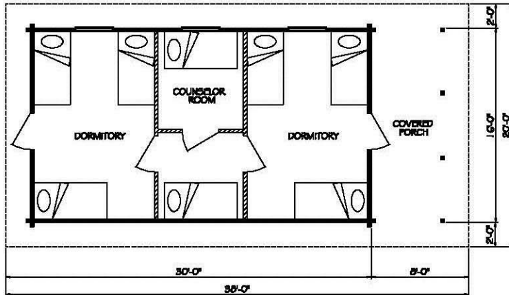
FLOOR PLAN
