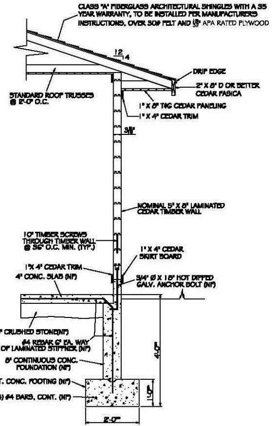
*** - DIMENSIONS TO SUIT LOCAL CODES TIMBER WALL CROSS SECTION
