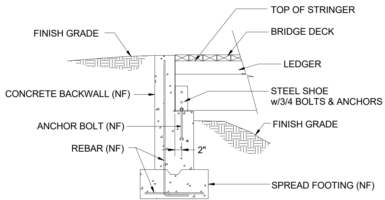
ABUTMENT CROSS SECTION FINAL SIZE TBD
