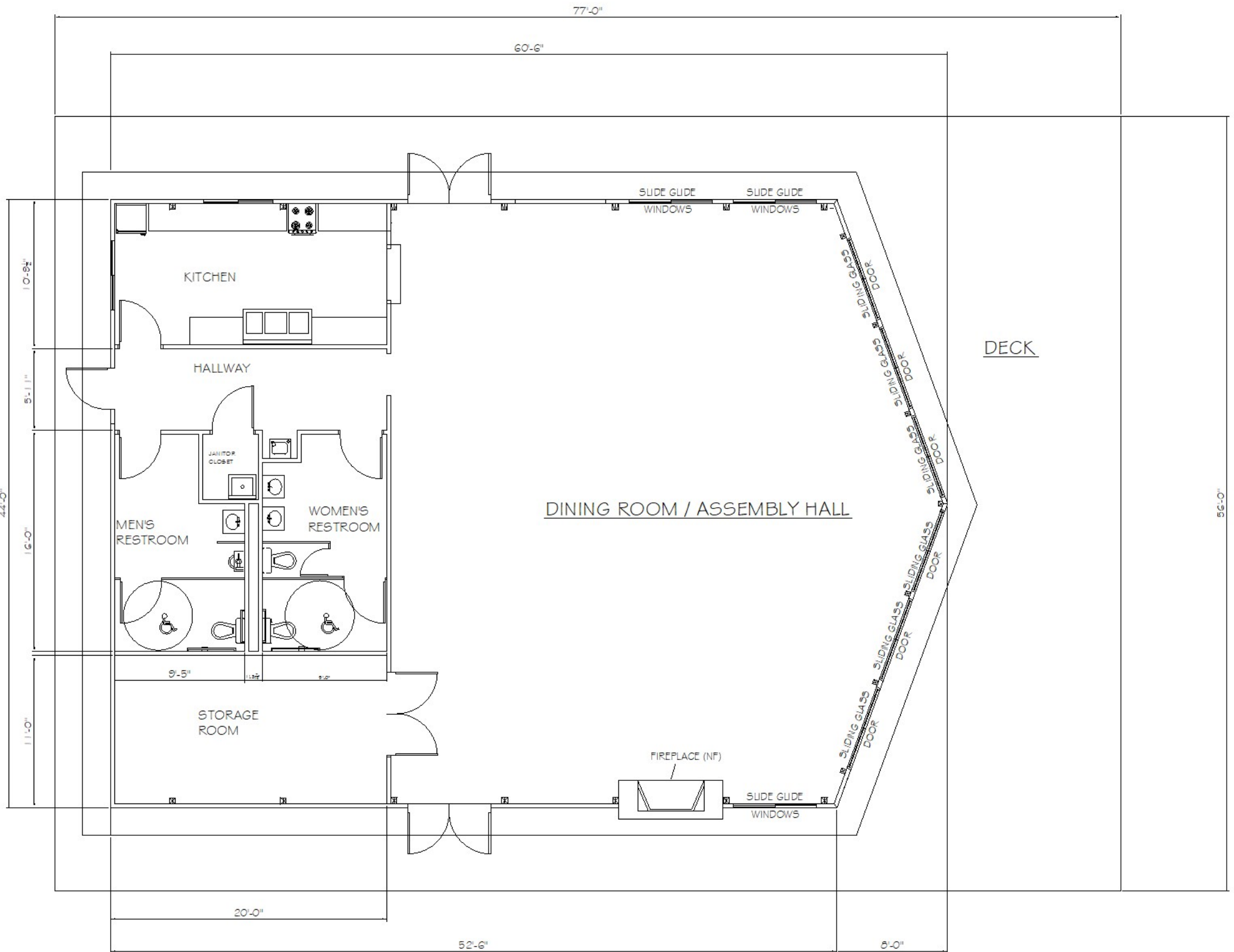
FLOOR/ROOF PLAN SCALE: 1/4" = 1'-0"
